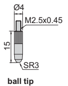
ball tip
