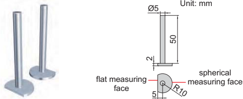
Measuring external groove diameter with flat measuring face (depth h1 \leq 2.5\text{mm} )
