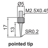
pointed tip
